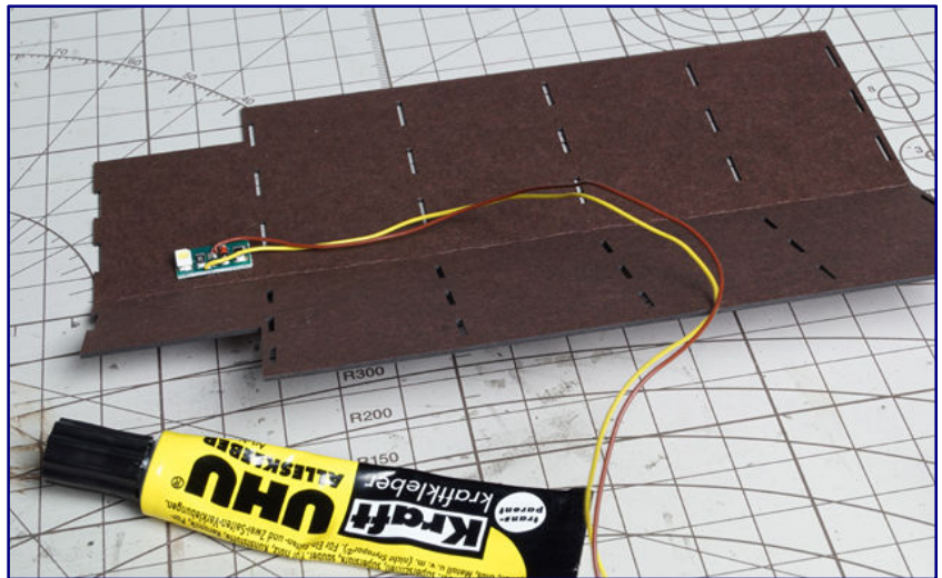
We glue an LED board (Viessmann 6008) almost centrally under the inner roof skin so that it radiates downwards.
